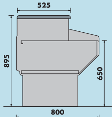
ATENA MESA TERMINAL ATENA CASH DESK
