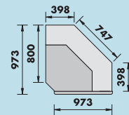
MESA TERMINAL - ÂNGULO EXTERNO 90° CASH DESK - 90° EXTERNAL CORNER
